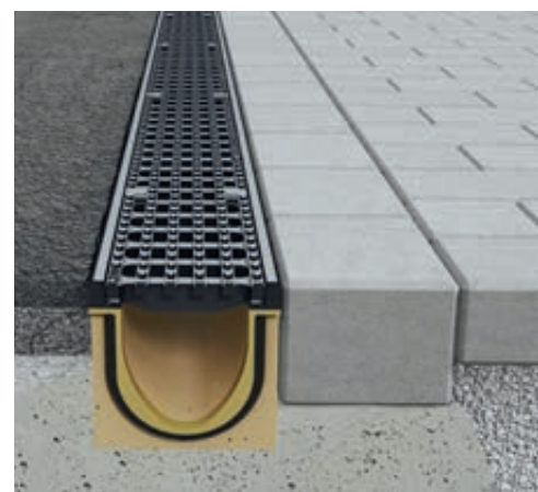
Surface covering directly worked in: ACO DRAIN® Multiline HD Seal in with cast frame
