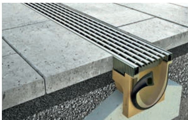
ACO DRAIN® Multiline Seal in frame steel, galvanised or stainless steel
