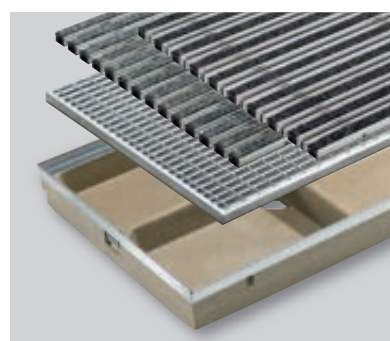
Vario floor tray with steel frame for all shoe scraper mats and Vario step-on gratings
